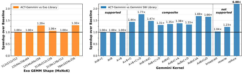
Fig. 21. Speedup of compiled code by ACT-Gemmini over Exo library (left) and Gemmini SW library (right). Note that the “not supported” evaluation (right) is a cross-architecture comparison: these operators have no Gemmini implementation in the SW library, so the baseline numbers were measured against the host CPU.
