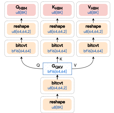
Fig. 9. The initial e-graph for G_{QKV} [after Module 1]. G_{QKV} (Fig. 4) is not expanded here for compactness.
